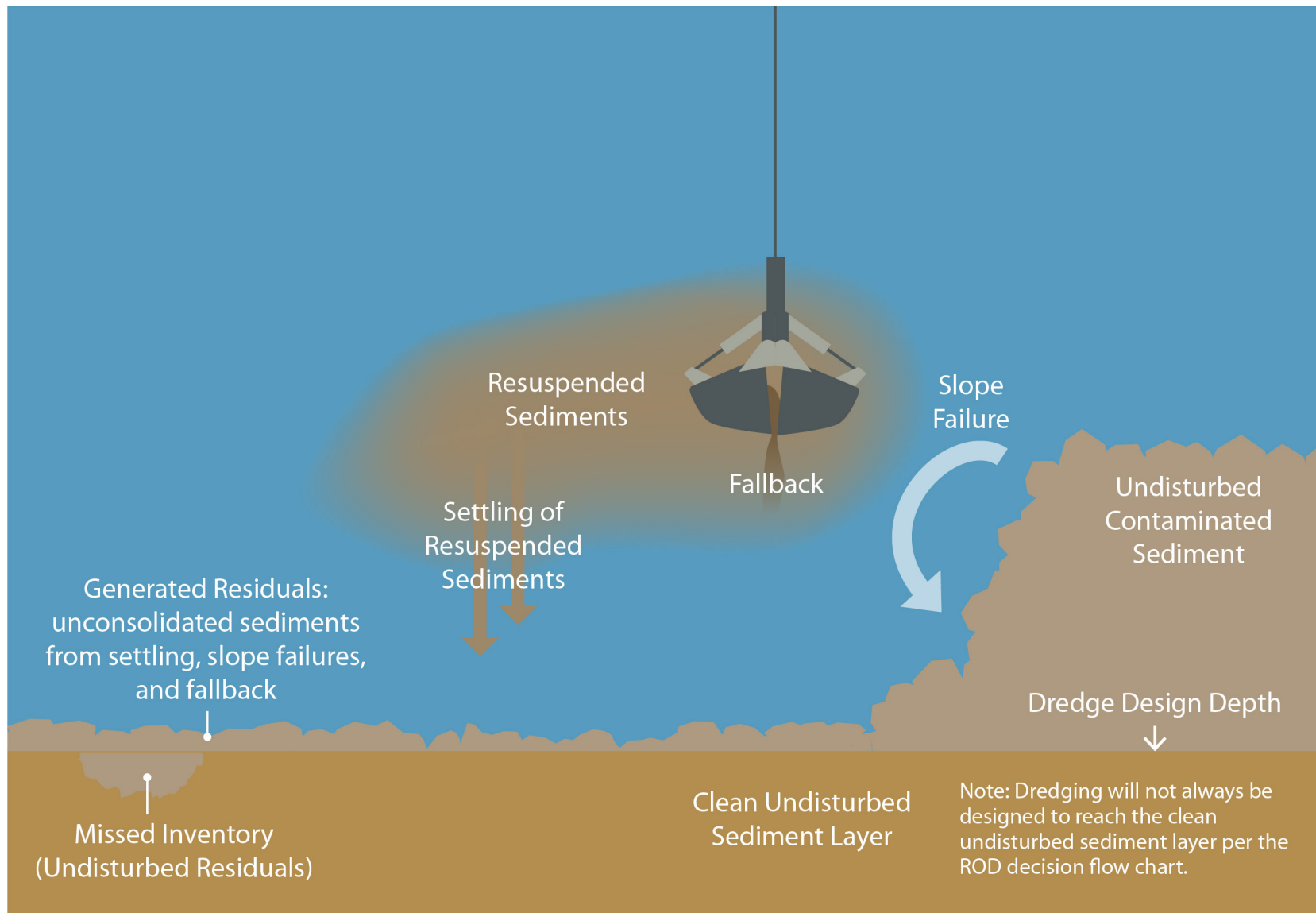
Figure 3-2. Dredge Residuals Schematic REMEDIAL DESIGN WORK PLAN FOR LDW MIDDLE REACH
