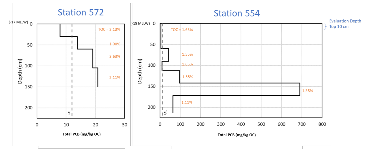
Figure Q-1 Sediment Profiles of Cores 572 and 554
