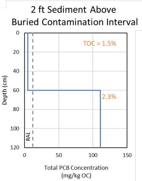
Figure Q-3 Generalized Core Profile for RAAs 14 and 15
