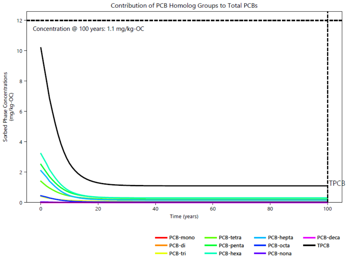
Figure Q-5 Temporal Profile of Model-Predicted PCB Concentrations Within the Top 10 cm of Sediment, Assuming Sedimentation
