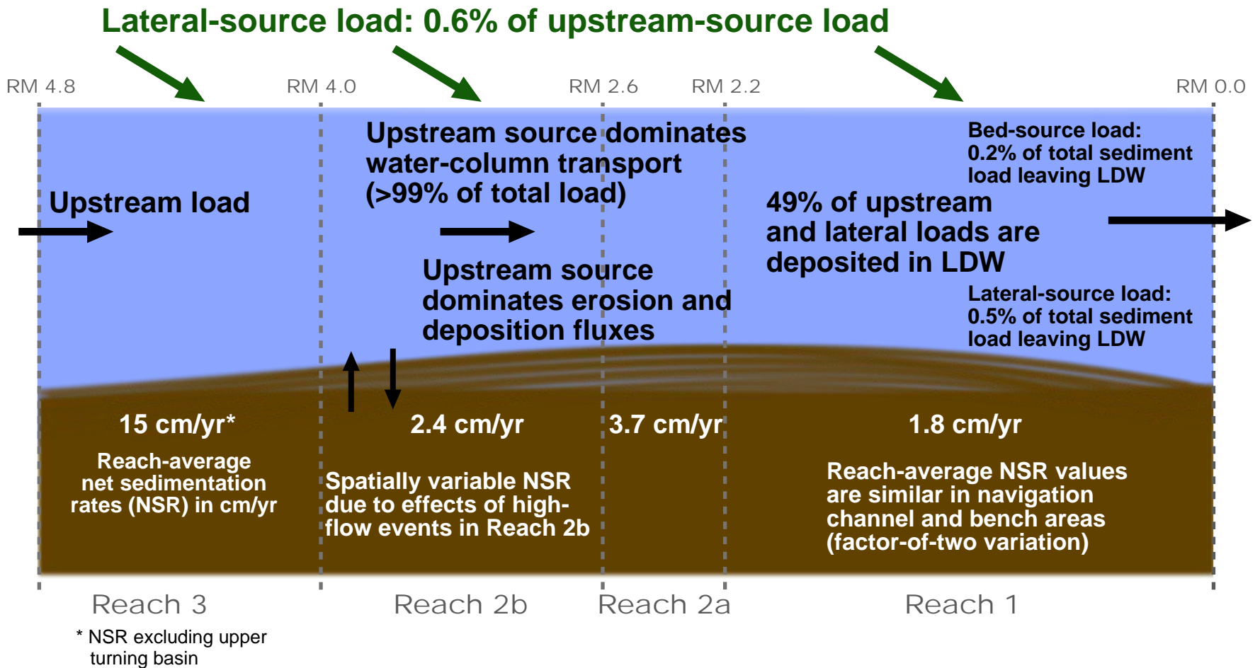
Figure 5-4. Schematic of LDW sediment transport processes during 30-year period. Upstream load is sum of suspended load and bed load.
