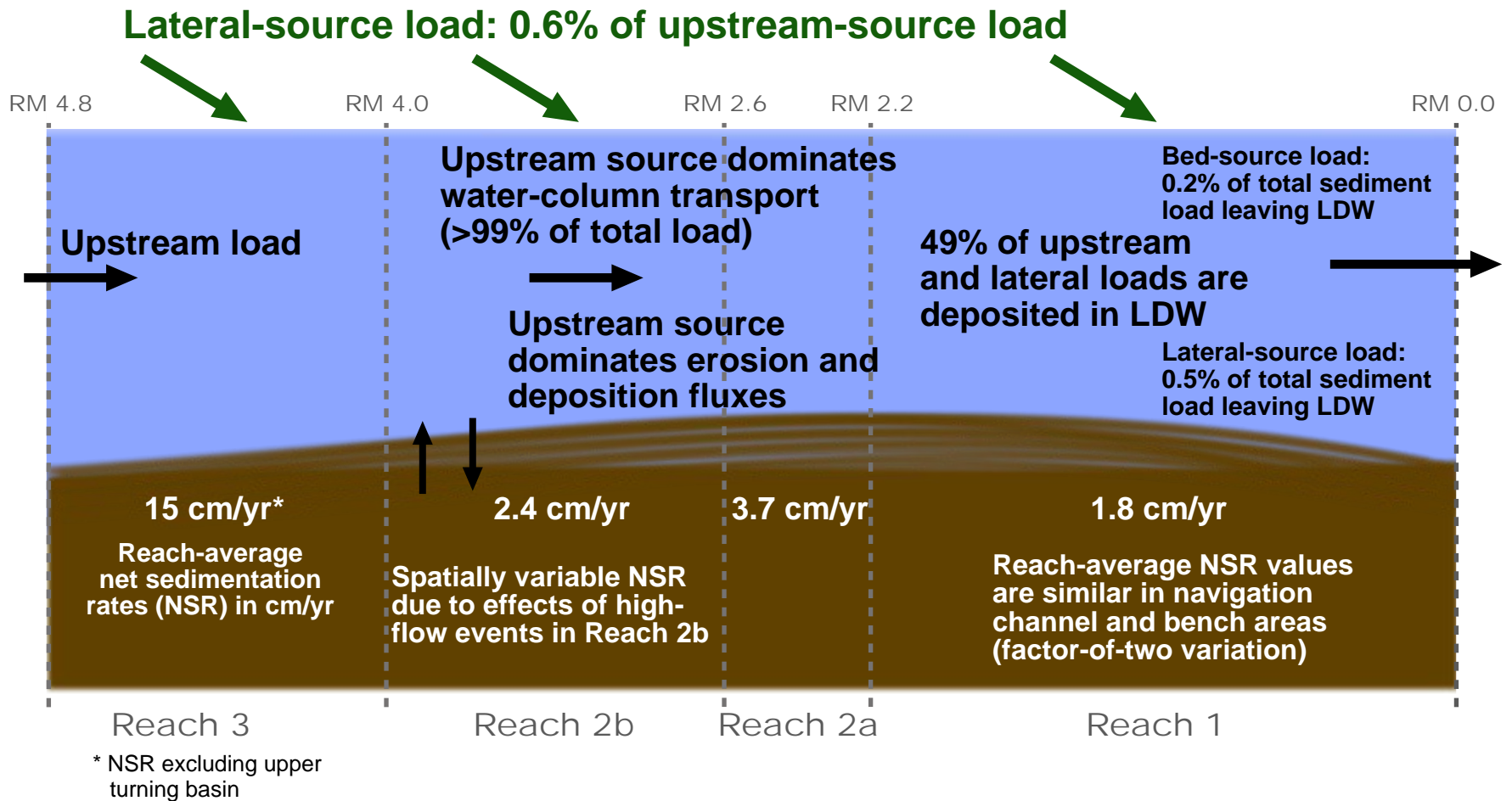
Figure ES-4. Schematic of LDW sediment transport processes during 30-year period. Upstream load is sum of suspended load and bed load.
