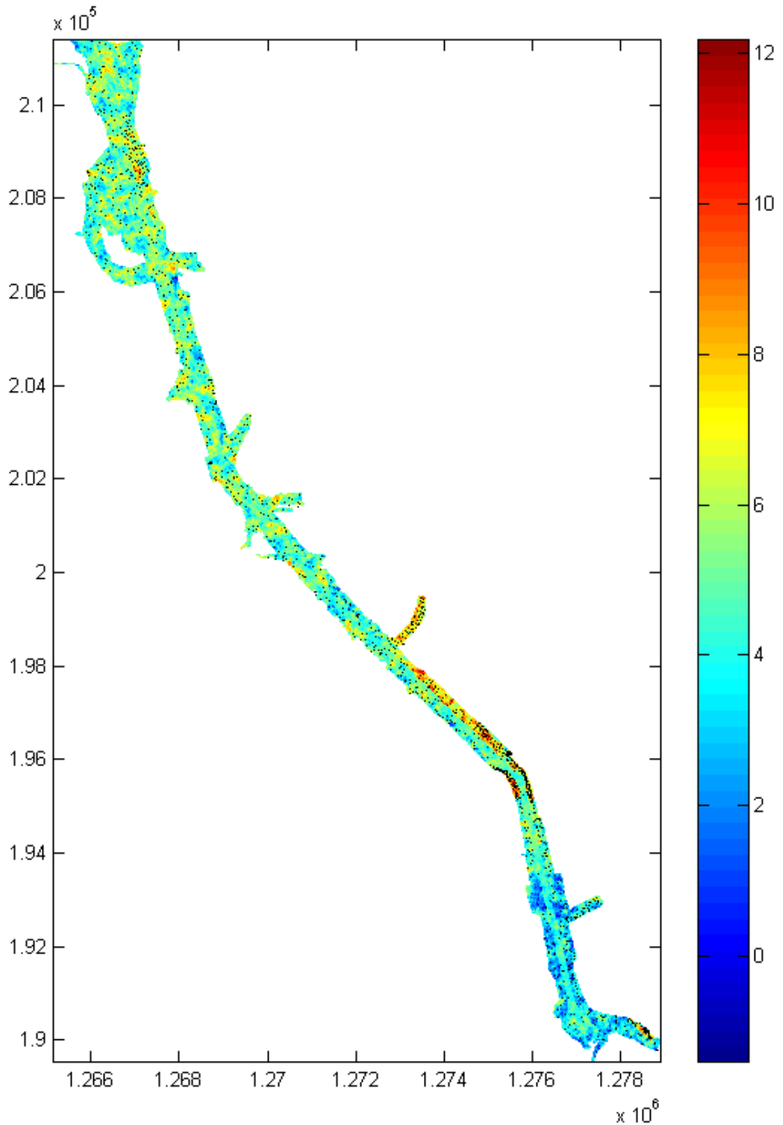
Figure 5. Simulated log(PCB) concentration in surface sediments. One of 1000 realizations generated. Black dots represent sample locations.
