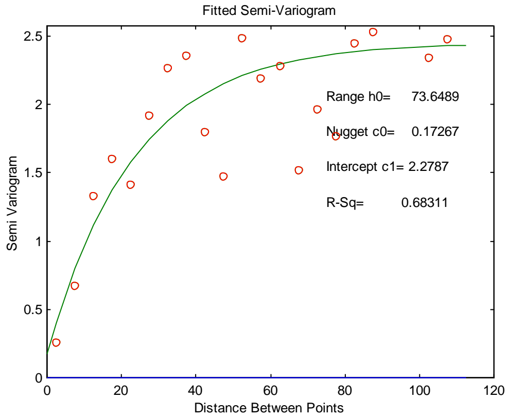
Figure 3. Semivariogram of residual log(PCB) concentration.
