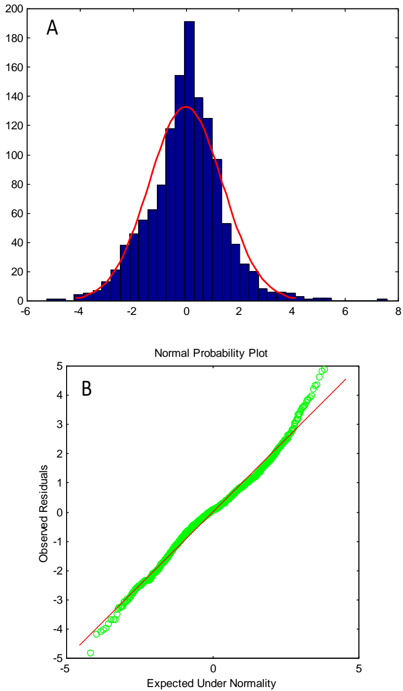
Figure 2. Histogram of residuals of log(PCB) with fitted normal distribution (panel A) and normal probability plot for residuals (panel B). Residuals are similar to a normal distribution ( p > 0.10 )
