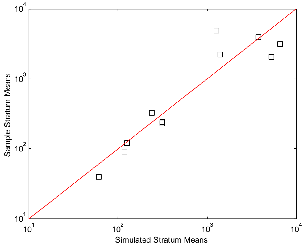
Figure 4. Sample vs. simulated stratum means from one synthetic population.
