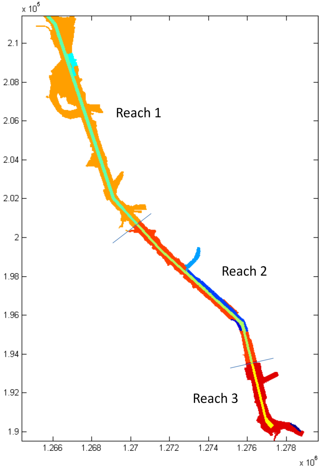
Figure 1. Stratification of study area in the Lower Duwamish Waterway Site.
